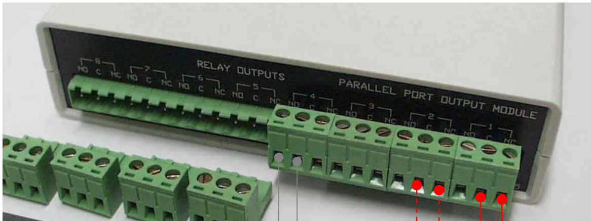
For lights power use NO - C
